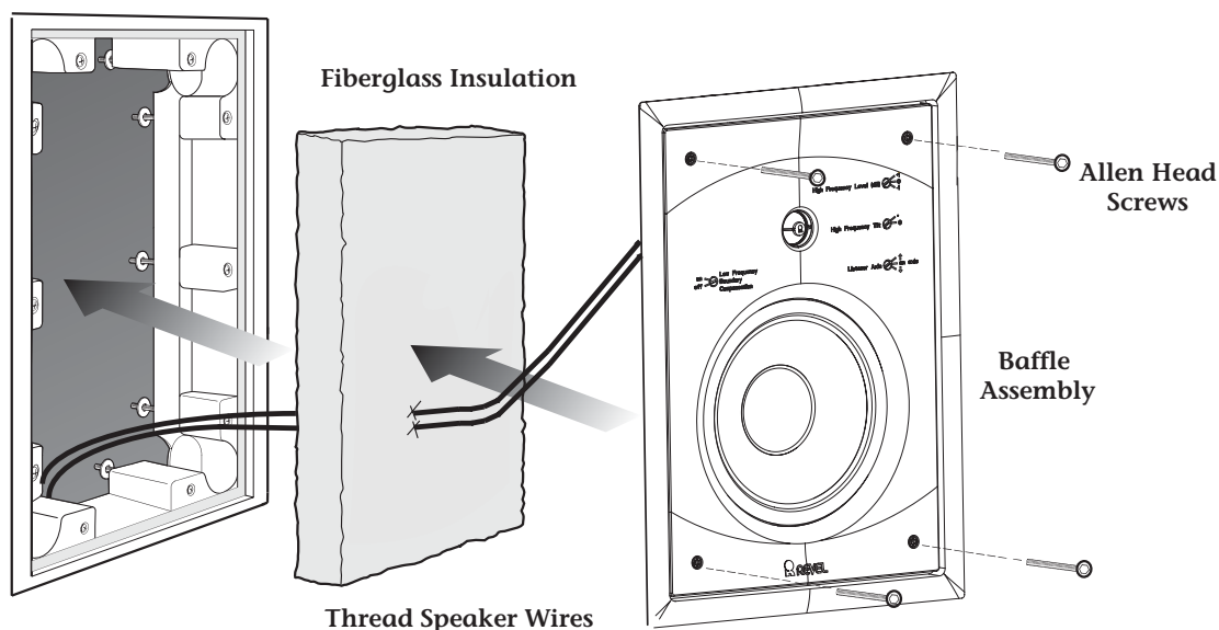
Figure 16: Install the Insulation and Baffle
