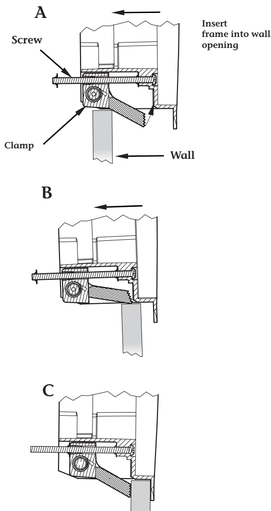
Figure 14: Clamp Mechanism
