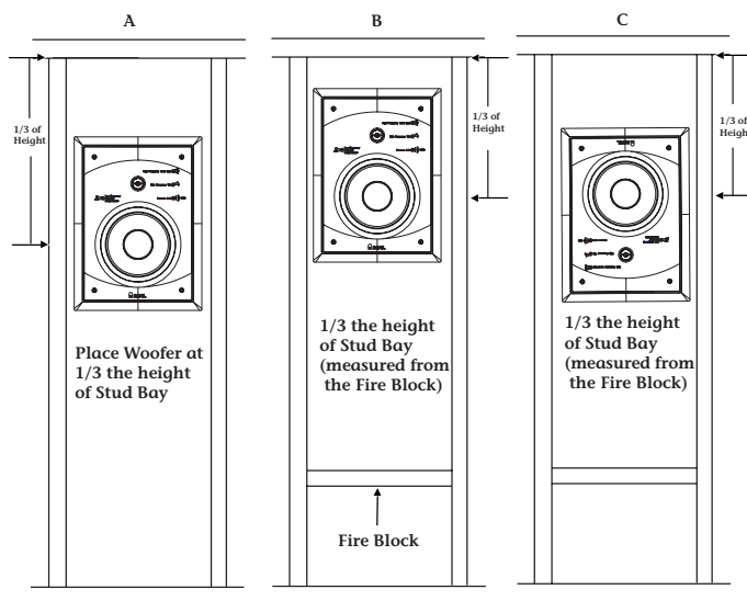
Figure 11: Ideal Height of Woofer
