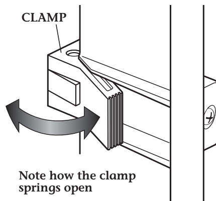
Figure 13: Clamp Closeup
